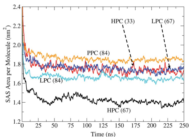
Fig. 5 Solvent-accessible surface area per molecule as a function of time for the five AT simulations indicated in the plot. Data were progressively averaged over 0.5 ns for clarity.
