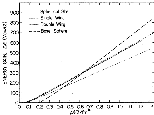
FIG. 3. Energy drop -\Delta\epsilon in Ali-Bodmer alpha matter for four different abnormal occupations, extended to higher densities (see Fig. 2).
