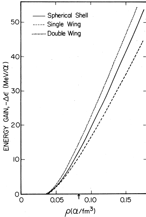
FIG. 2. Energy lowering -\Delta\epsilon in Ali-Bodmer alpha matter for single-wing, double-wing, and spherical-shell abnormal occupations, relative to the energy for normal occupation. (The energy drop is maximized, at each density \rho , with respect to the free parameters in the assumed momentum distribution.) The vertical arrow marks the equilibrium density of alpha matter obtained in Ref. 21.
