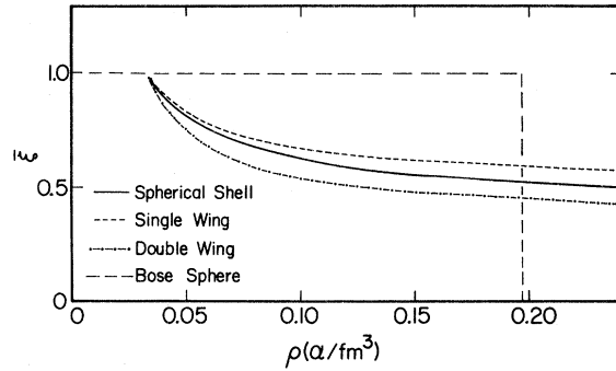
FIG. 4. Optimal zero-momentum condensate fraction \bar{\xi} in Ali-Bodmer alpha matter, corresponding to minimization of the energy, at each density, with respect to the free parameters of the assumed abnormal momentum distributions.
