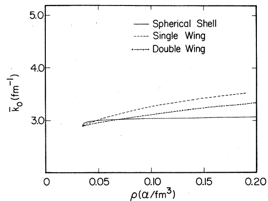
FIG. 5. Optimal value \bar{k}_0 of parameter k_0 (or k_B in the Bose-sphere case) in Ali-Bodmer alpha matter, corresponding to minimization of the energy, at each density, with respect to the free parameters of the assumed abnormal momentum distributions.
