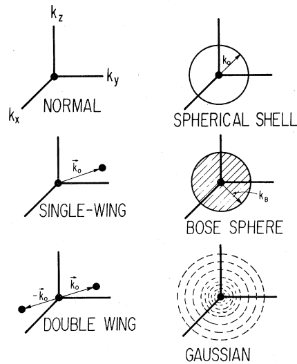
FIG. 1. Schematic representation of various abnormal occupations investigated in this paper, compared to the normal one.
