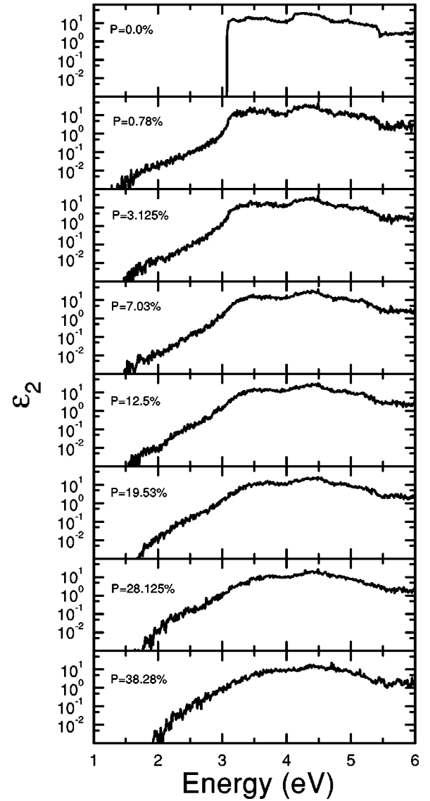
FIG. 4. Showing the low-frequency tail of the imaginary part of the dielectric function, \varepsilon_2(\omega) , as a function of photon energy for different porosities. The calculations were performed using 225 \mathbf{k} points in the Brillouin zone.
