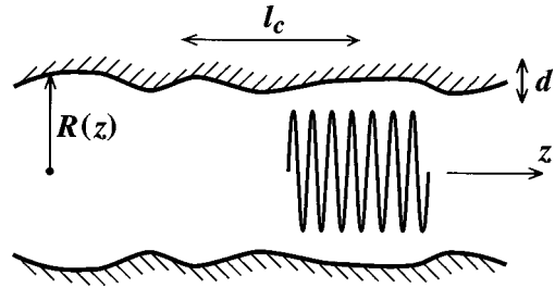
FIG. 6. The geometry of an undulating wire. The fluctuations of the radius of the wire are small compared to R_0 and they are smooth on the electron wavelength.
