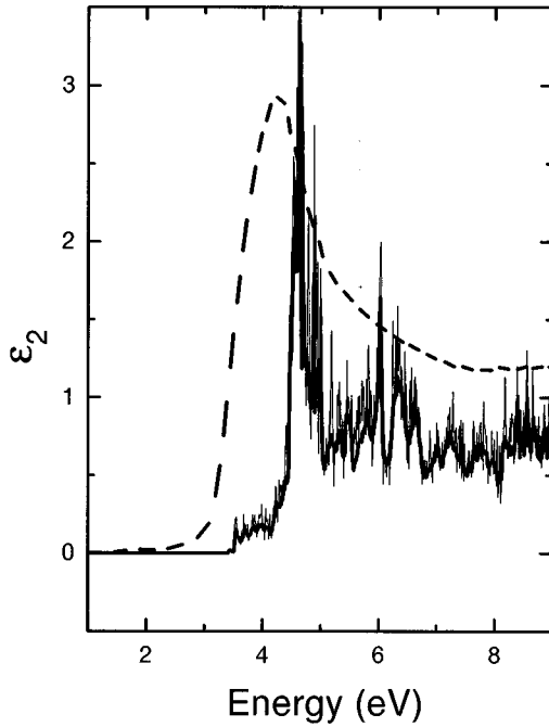
FIG. 5. Comparison of the experimental dielectric function for 70% porous Si (dashed line) with our calculations for the 128-atom supercell model at 76% porosity. The thin-solid line represents the response in the perfect case (vertical optical transitions), and the smoothening of the curve by disorder (vertical and nonvertical transitions) is given by the thick-solid line (see text). The experimental data are presented by digitizing the plot of Ref. 14.
