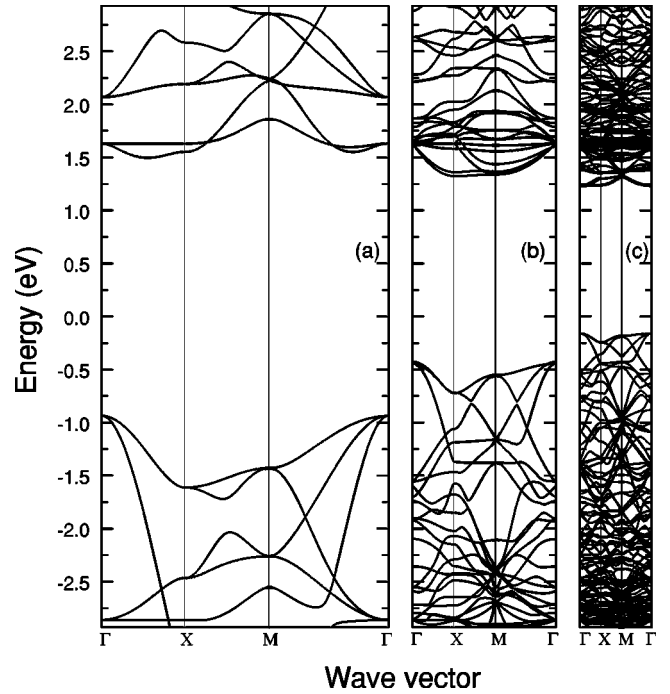
FIG. 2. Showing the band structure for por-Si of porosity 12.5%, using (a) an 8-atom supercell (with 1 atom removed), (b) a 32-atom supercell (with 4 atoms removed), and (c) a 128-atom supercell (with 16 atoms removed).
