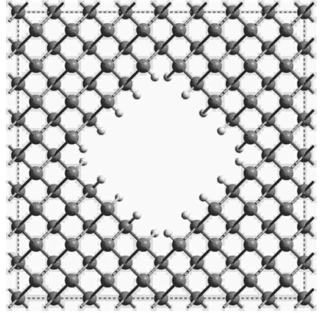
FIG. 1. Showing the 128-atom supercell with 25 Si atoms removed (19.53% porosity). The surface of the pore is saturated with hydrogen atoms, and por-Si is modeled by repeating this sort of supercell periodically.
