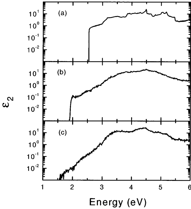
FIG. 3. Imaginary part of the dielectric function, \varepsilon_2(\omega) , versus the photon energy for the same cases as in Fig. 2. (a) An 8-atom supercell (with 1 atom removed), (b) a 32-atom supercell (with 4 atoms removed), and (c) a 128-atom supercell (with 16 atoms removed).
