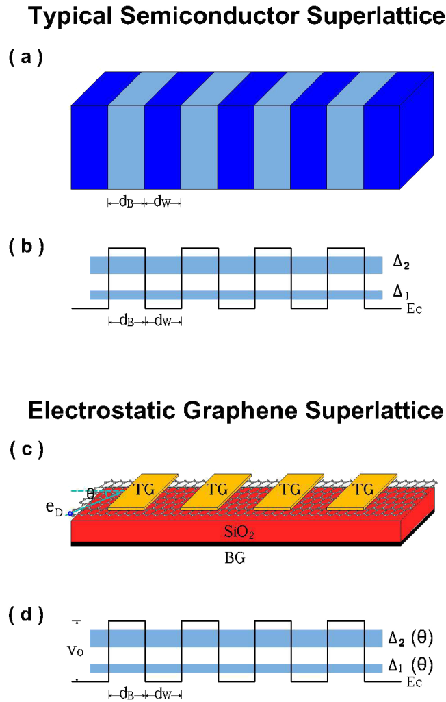
FIG. 1. Schematic representation of Typical Semiconductor and Electrostatic Graphene Superlattices. The cross-sections of these superlattices are shown in (a) and (c), while in (b) and (d) the conduction band-edge profiles and the energy minibands ( \Delta_1 and \Delta_2 ) of them are depicted. d_B , d_W and V_0 represent the widths of barriers and wells, and the height of the barriers, respectively. Aside to the structural differences, the main physical difference is that energy minibands and gaps in the case of Electrostatic Graphene Superlattices depend on the angle of incidence.
